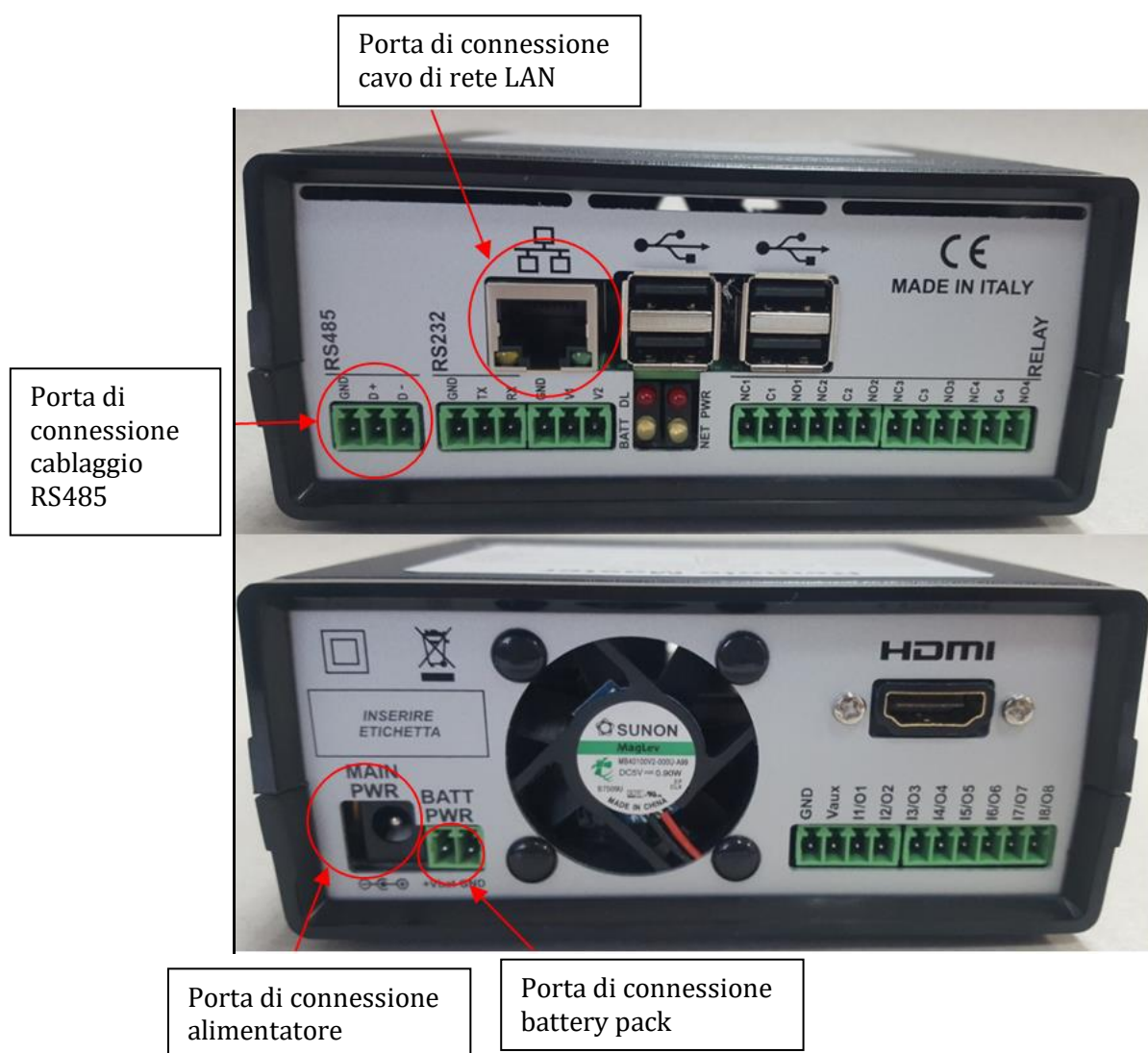
Figura108: Back Datalogger
